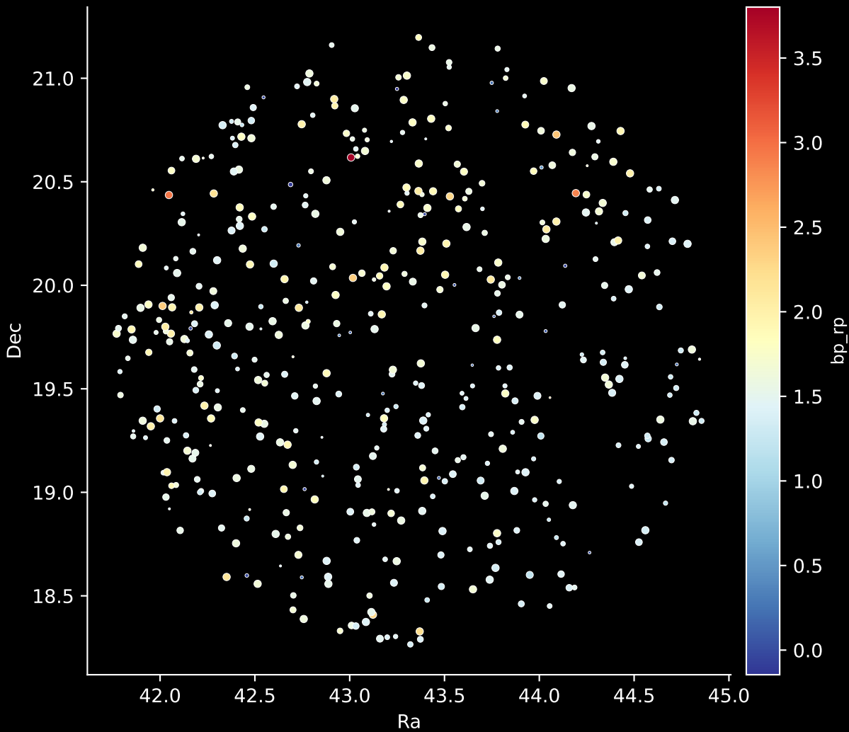
APOGEE DR17 Field: [060-08] Stars: 458
