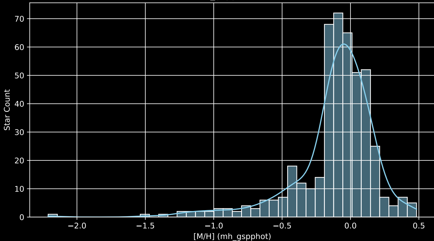
APOGEE DR17 Field: [060-08 [M/H] (mh_gspphot) (n= 455)
