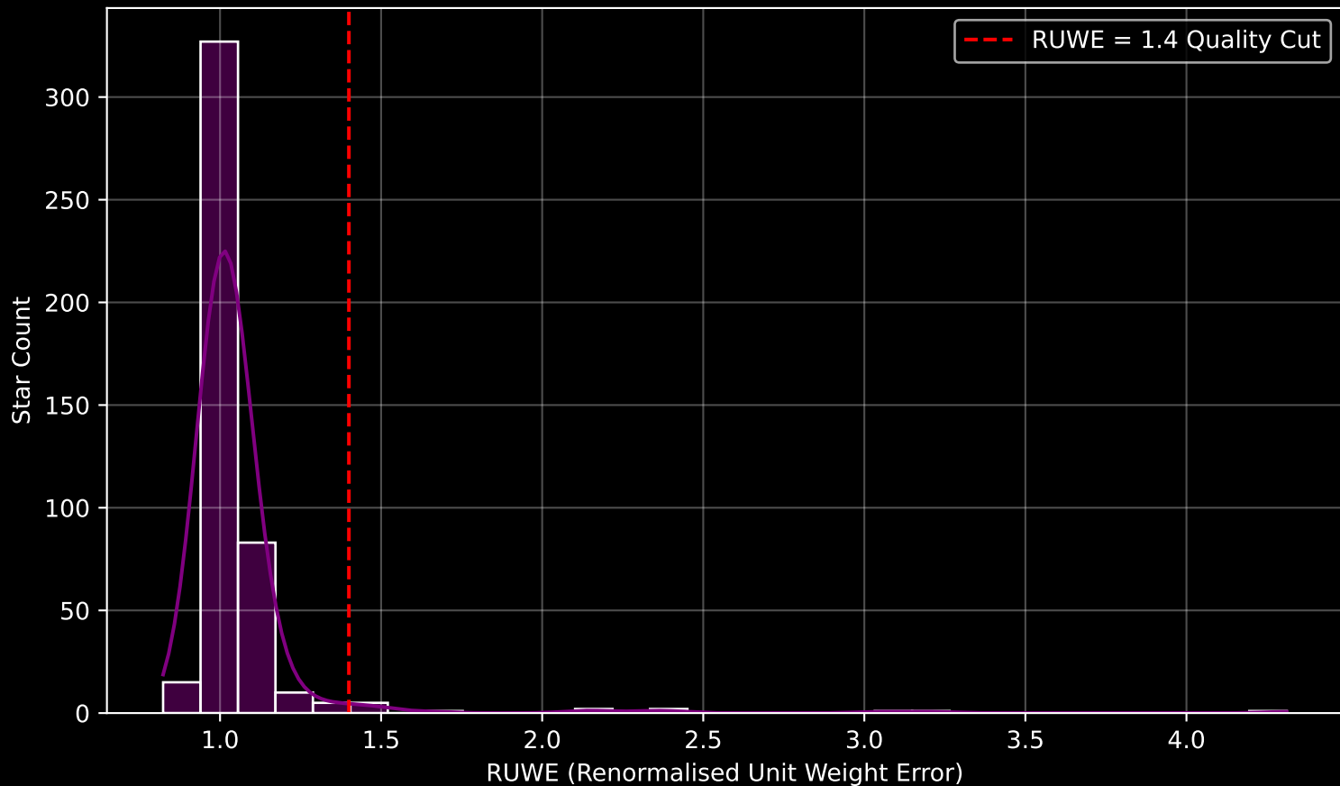
GAPOGEE DR17 Field [060-08] RUWE Distribution (n= 453)
