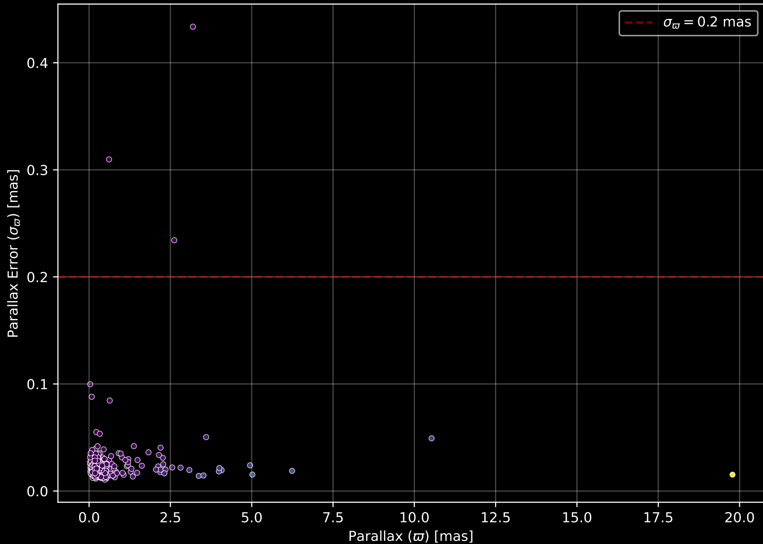
APOGEE DR17 Field: [060-08] Parallax Quality (n= 458)
