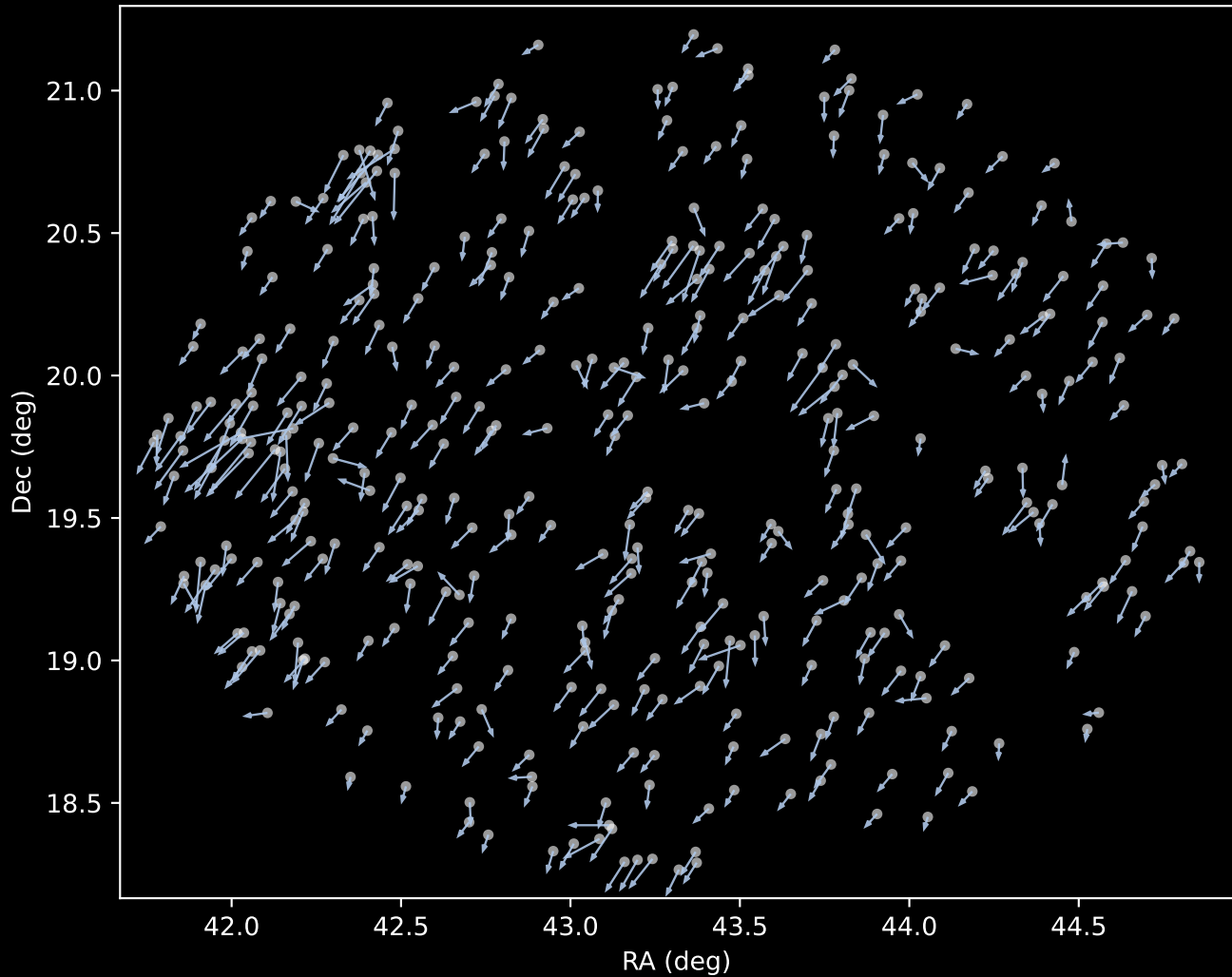
APOGEE DR17 Cluster 1 Proper Motion Vectors (n=392)
