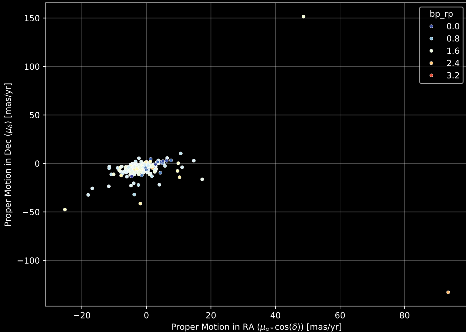
APOGEE DR17 Field: [060-08] Proper Motion Diagram (n= 458)
